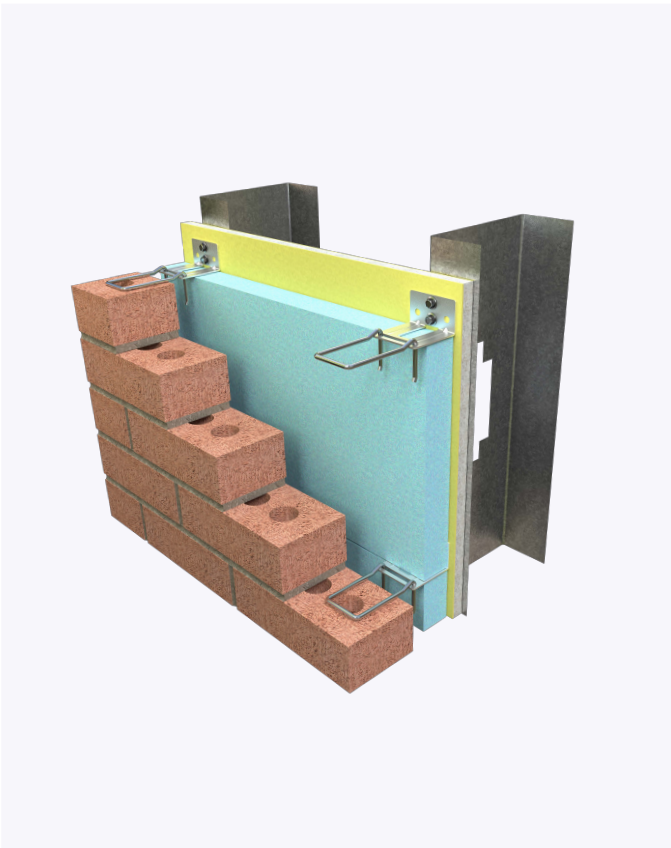
***Anchor can be installed Horizontal or Vertical.***
