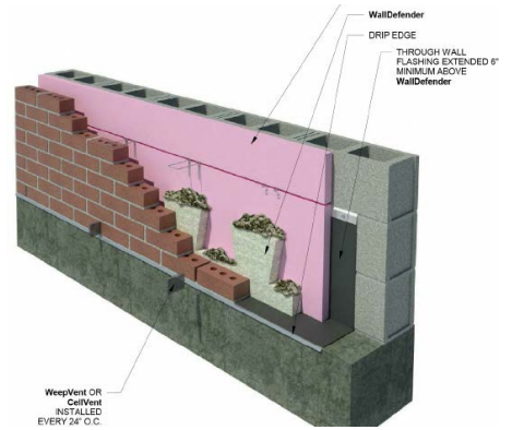
Wall Base Detail
